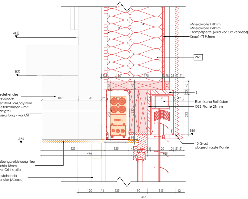
Detail 11 - PT-1
