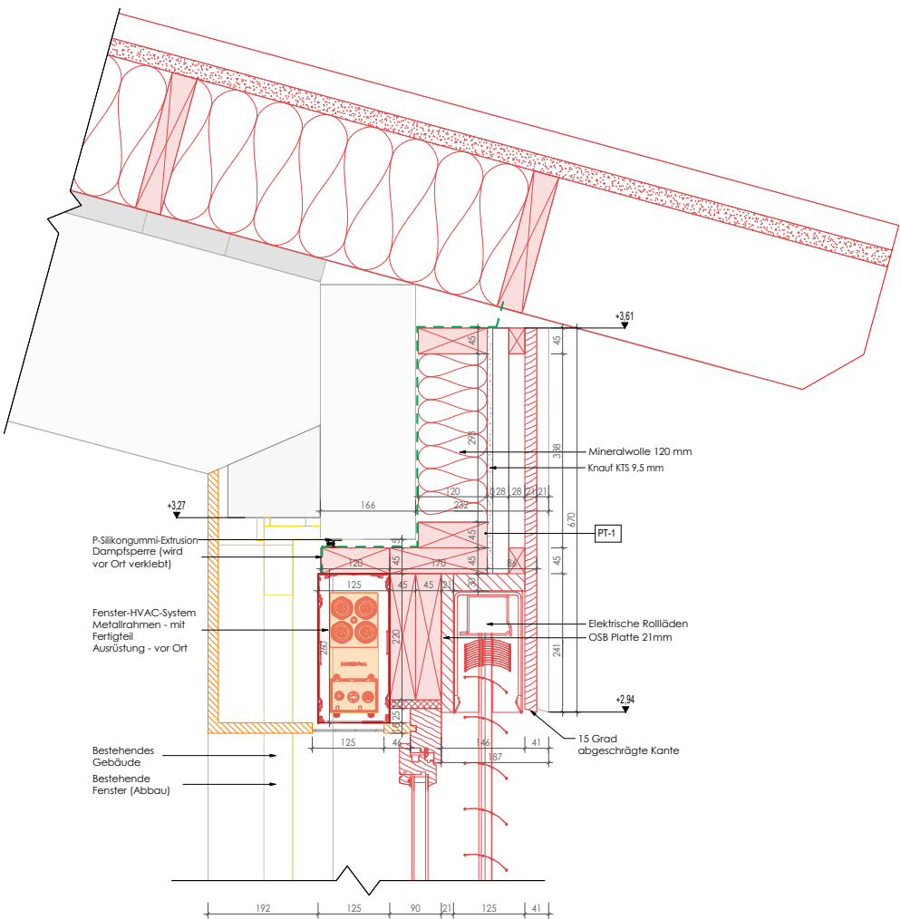
Detail 10 - PT-01
